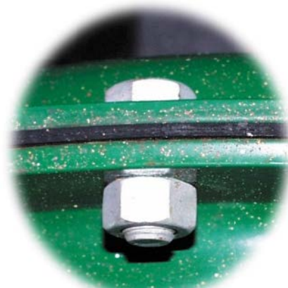
Powder-Coated Actuator Casings with NCF Coated Cap Screws after One Year of Service on an Off-Shore Platform (Light-Colored Spots are Paint Drift from Customer Paint Spraying of Nearby Equipment)
